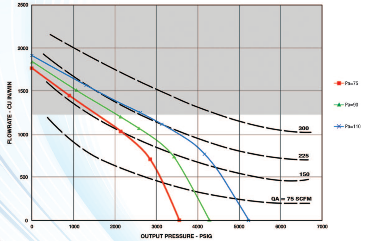
8SFD2-55 PERFORMANCE
