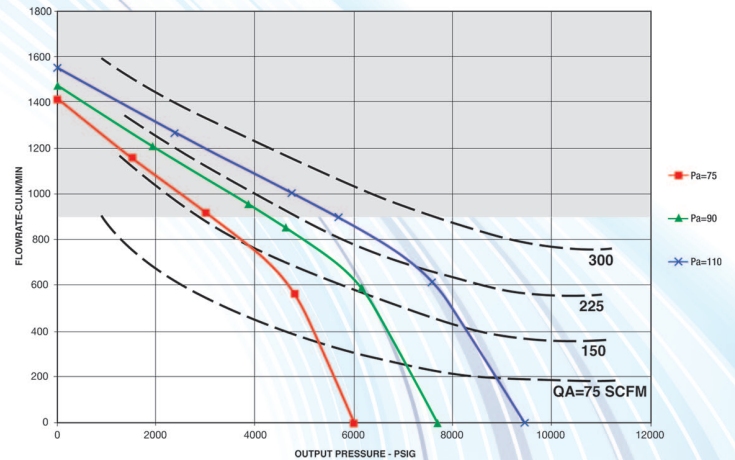
8SFD2-88 PERFORMANCE
