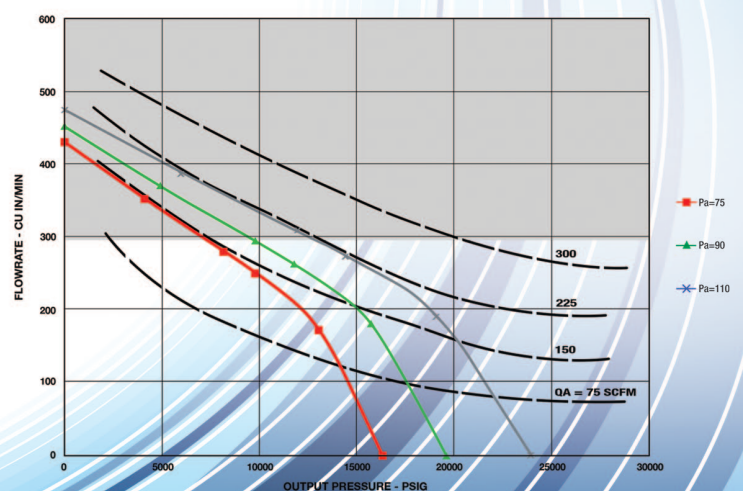
8SFD2-224 PERFORMANCE
